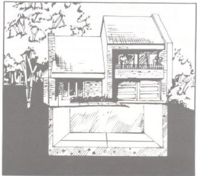
Eliminate Entry Routes for Soil Gases by Proper Jointing, Sealing, and (When Necessary) Venting.
