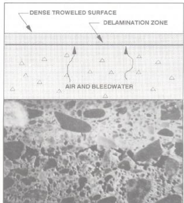
Delaminated Concrete
