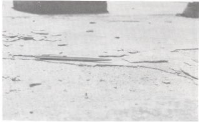
Delaminated Concrete
